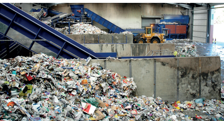
Photo: Mechanical recycling plant
